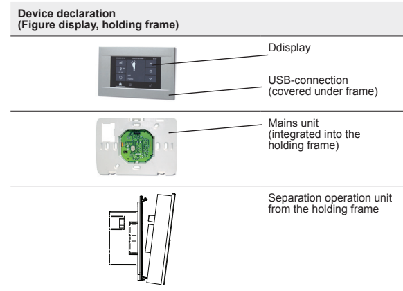
Fig. 1 Device views
